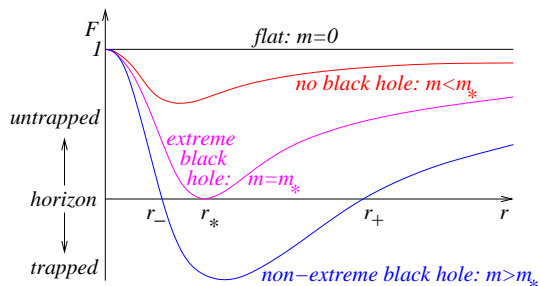
FIG. 2: The metric function F = g^{rr} , whose sign determines gravitational trapping, for fixed core radius l and different total masses m .
