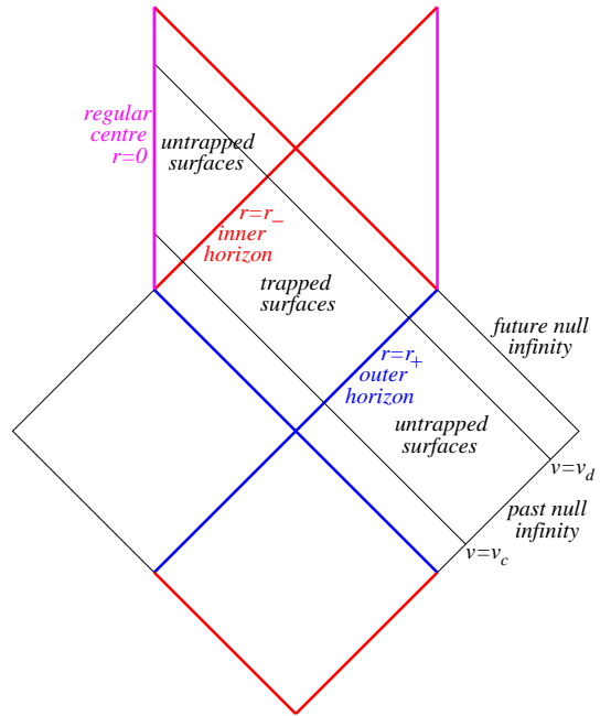
FIG. 1: Penrose diagram of a regular non-extreme black hole, to be identified vertically with isometric regions.
