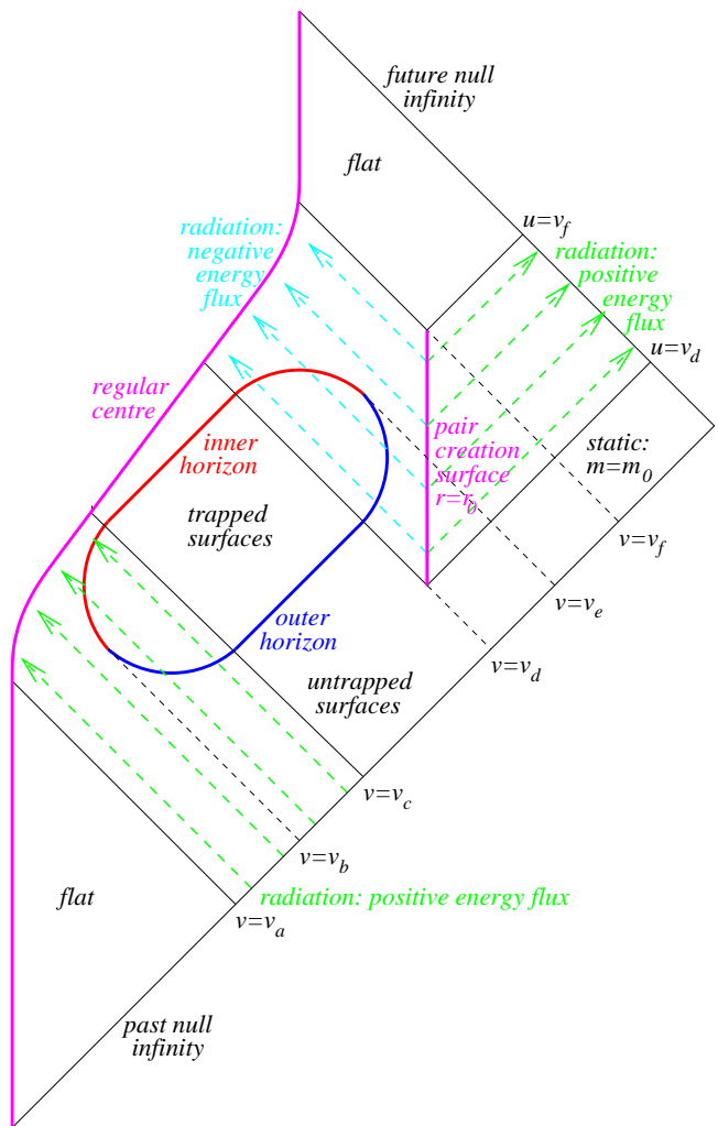
FIG. 5: Penrose diagram of formation and evaporation of a regular black hole in the given models.
